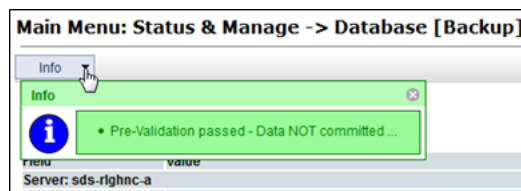
Figure 5-19 Verify Information
