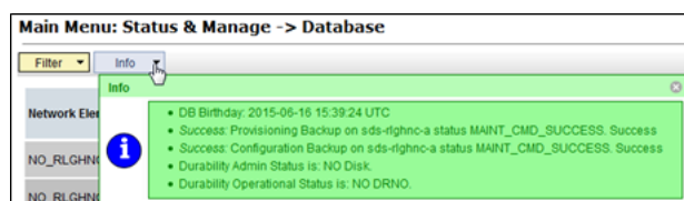
Figure 5-20 Provisioning Backup
