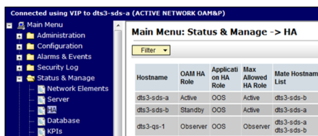
Figure 9-9 Filter
