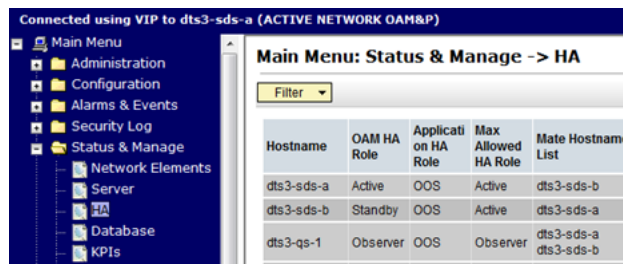
Figure 10-7 Filter
