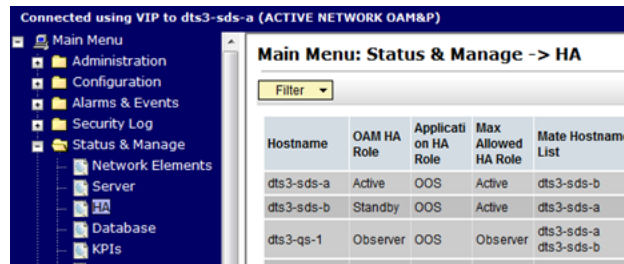
Figure 10-1 Filter
