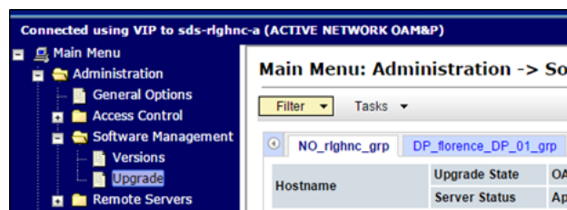
Figure 9-12 Upgrade
