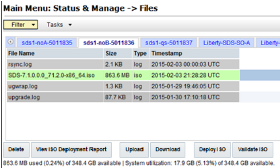
Figure 5-7 Deploy ISO
