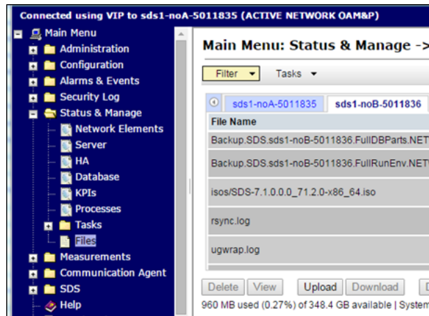
Figure 5-1 Upload
