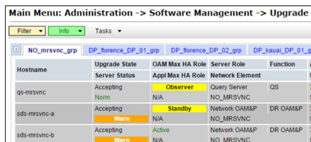
Figure 9-15 Upgrade State
