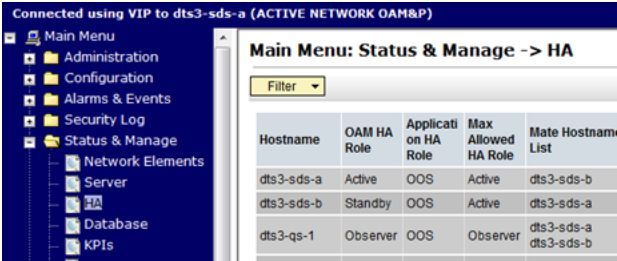
Figure 10-10 Filter
