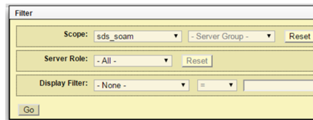
Figure 10-2 Scope
