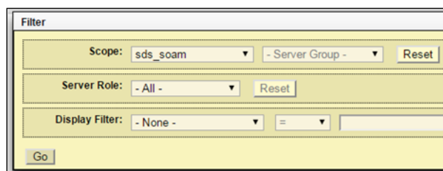
Figure 9-10 Scope
