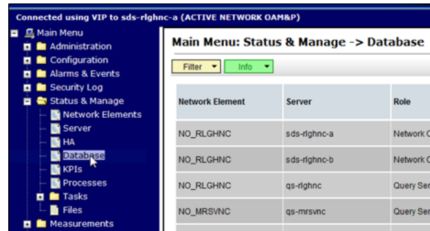
Figure 5-13 Database
