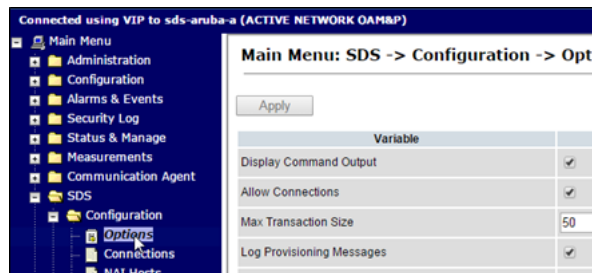
Figure 8-15 Options
