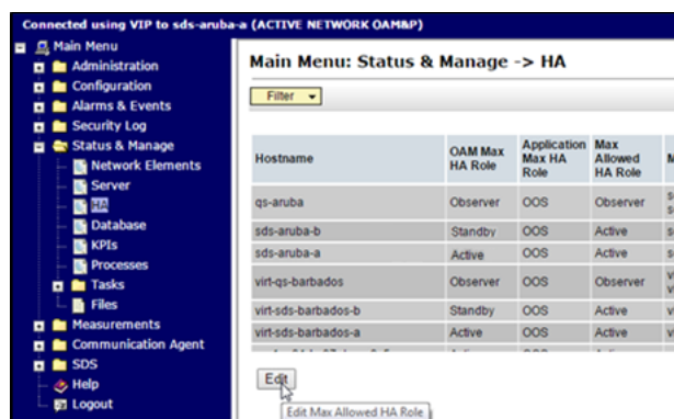
Figure 8-12 Edit Server
