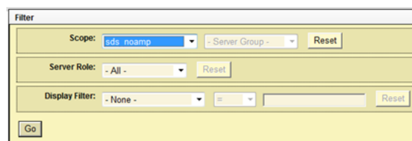
Figure 10-8 Scope
