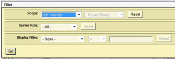
Figure 10-11 Scope
